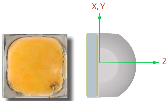
Figure 17: X, Y and Z axes in HD discrete LED ray files
